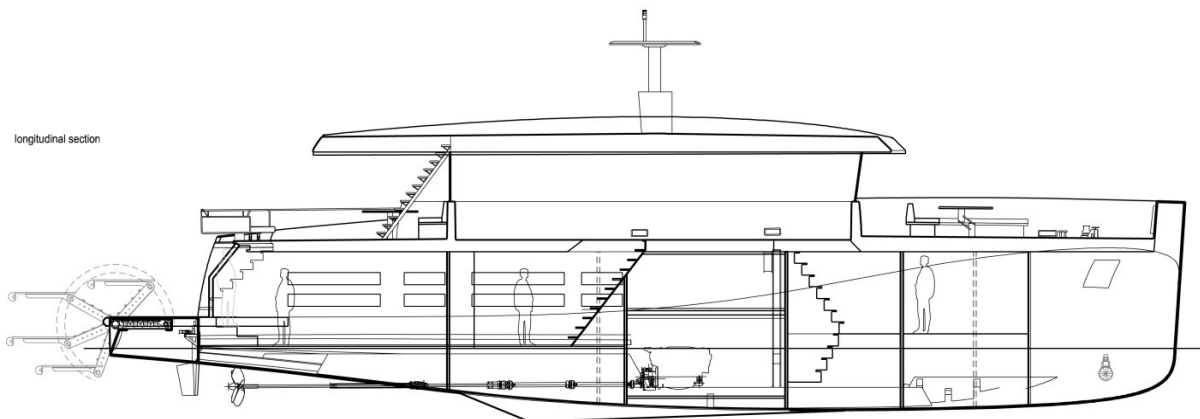
lower deck plan 3 cabin - A
